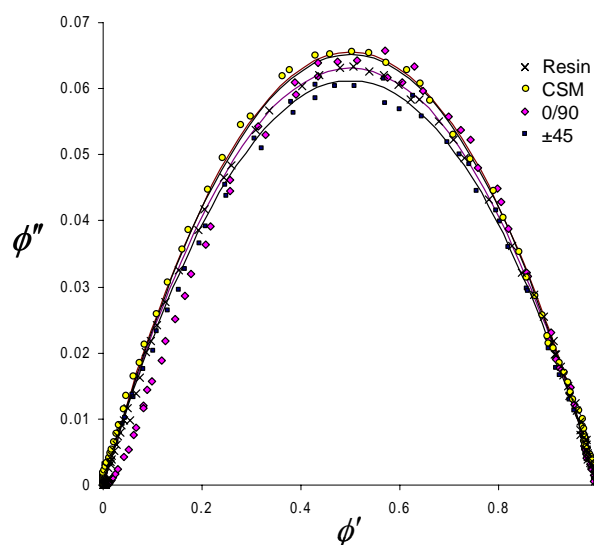
Fig 7. Cole-Cole plots for the DMTA data: pure resin ( \alpha = 0.160 ); CSM composite ( \alpha = 0.166 ); 0/90^\circ composite ( \alpha = 0.155 ), and \pm 45^\circ composite ( \alpha = 0.165 ).
