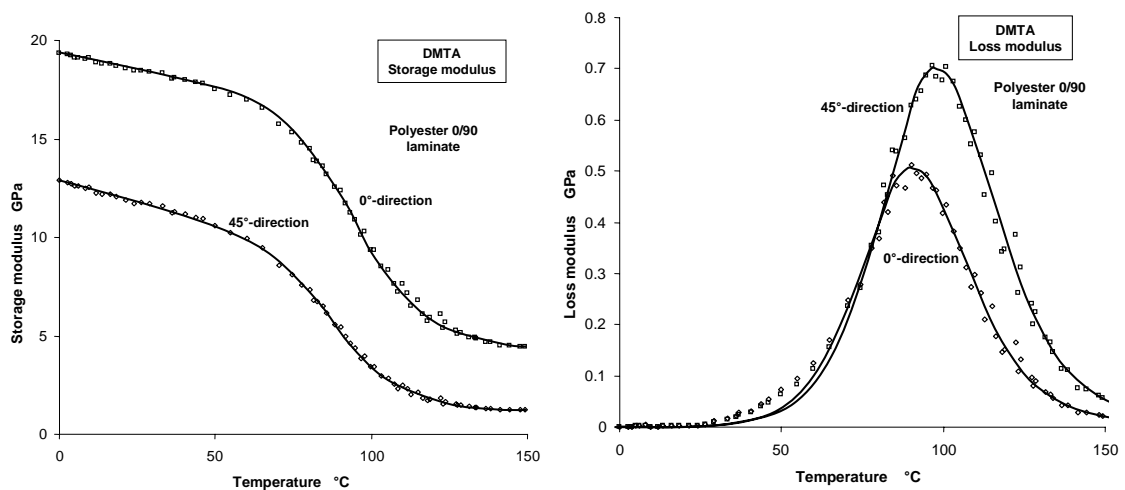
Fig 2. DMTA data (1 Hz, 10^\circ\text{Cmin}^{-1} ) for polyester/glass 0/90° laminate in the 0° and 45° directions. Continuous curves are C-C model fits, with parameters in Table 1.
