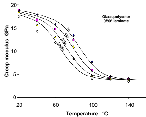
Fig 3. Flexural creep modulus in the 0° direction vs. temperature for glass/polyester 0/90° laminate. Continuous curves represent Cole-Cole model fit.
