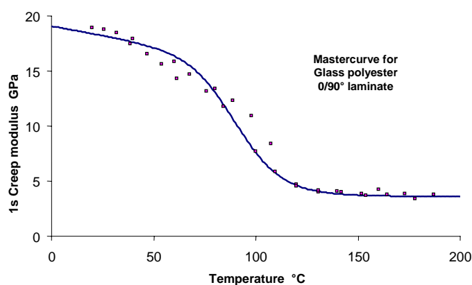
Fig 8. Flexural creep modulus in the 0^\circ direction vs. temperature for glass/polyester 0/90^\circ laminate. Master curve, shifted to 1s, for the data shown in Fig 3, fitted using the parameters from Table 1.
