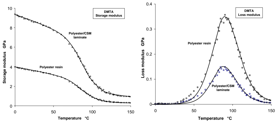
Fig 1. DMTA data (1 Hz, 10^\circ\text{Cmin}^{-1} ) for isophthalic polyester and for polyester-CSM composite. Continuous curves are C-C model fits, with parameters in Table 1.
