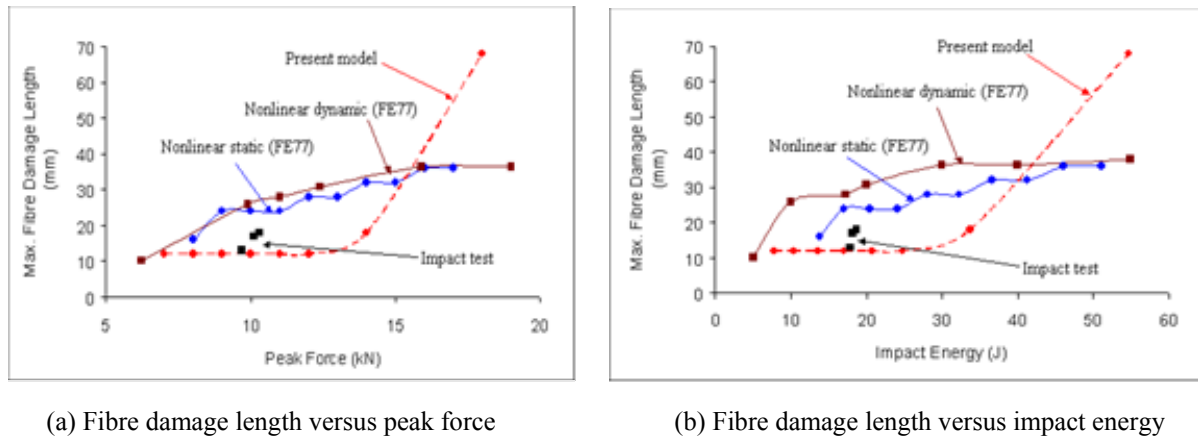
Fig. 7. Impact damage in an IM7/8552 ([45/-45/0/90] 3s ) circular plate. (a) Fibre damage length versus peak force and (b) Fibre damage length versus impact energy
