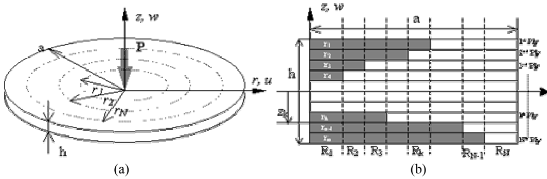
Fig. 1. Circular plate with fibre damage radius r_1, r_2, r_K, \dots, and r_N at each ply
