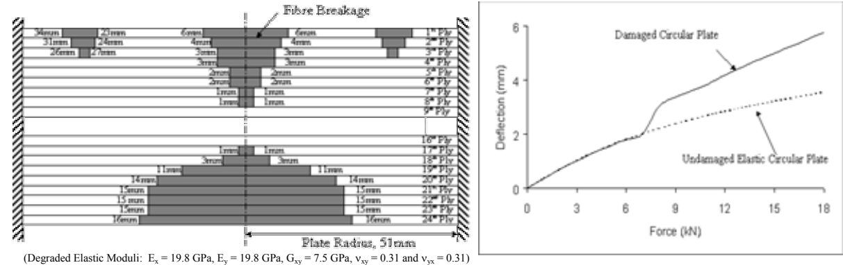
Fig. 5. (a) Through-thickness (Z-r plane) fibre damage in a 3mm thick [45/-45/0/90]_{3s} circular plate; applied load 18 kN and (b) central deflection versus applied force.
